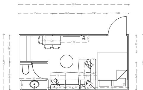
Tegola Caravan — Kitchenette · Bathroom · Lounge · Bedroom — Total 6,020mm × 3,090mm
