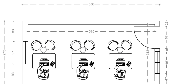
Foldable Caravan 1 — 3 Workstations — Total 5,880mm × 2,730mm
